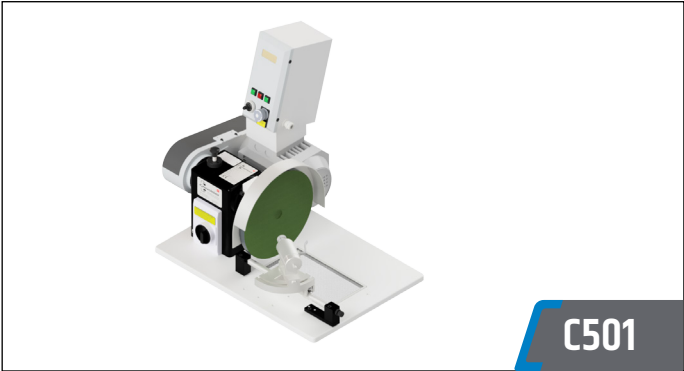
C501 machine in lapping configuration See the specific chapter for the accessories
