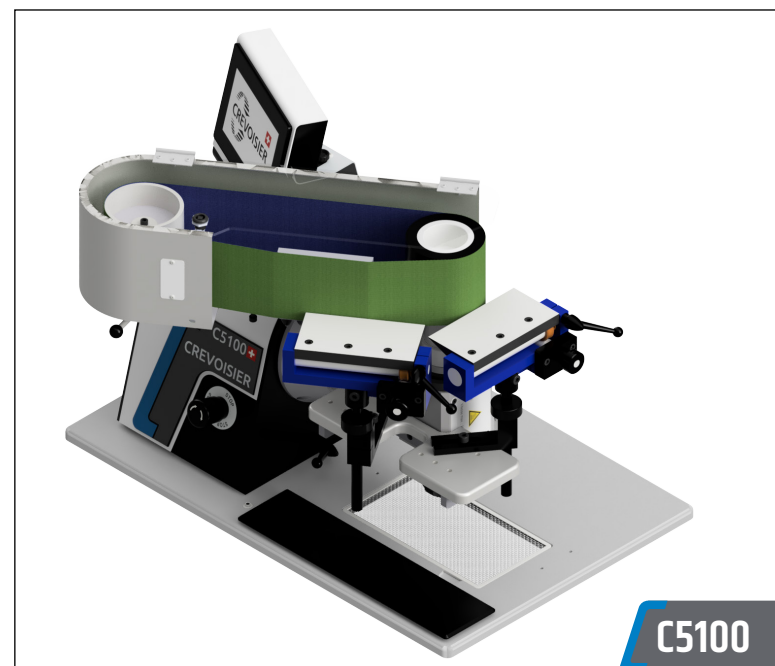
C5100 machine in horizontal satin-finishing configuration
