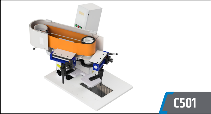
C501 machine in horizontal satin-finishing configuration See the specific chapter for the accessories
